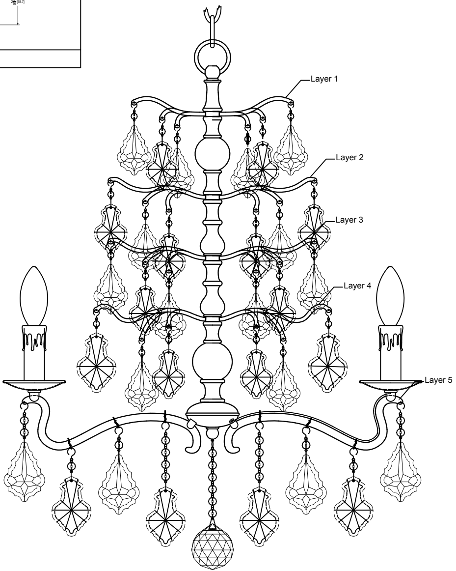
SECTION / ELEVATION
