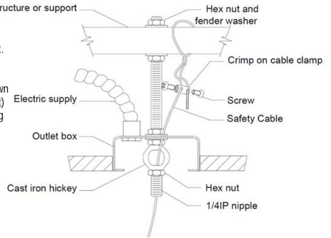
SUGGESTED FIELD CONSTRUCTED SUPPORT
