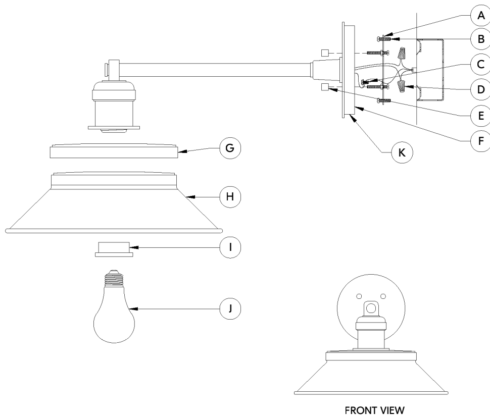
FRONT VIEW
