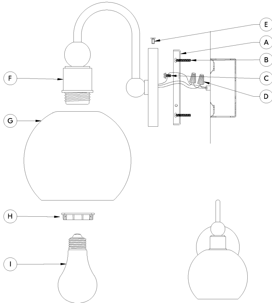
FRONT VIEW
