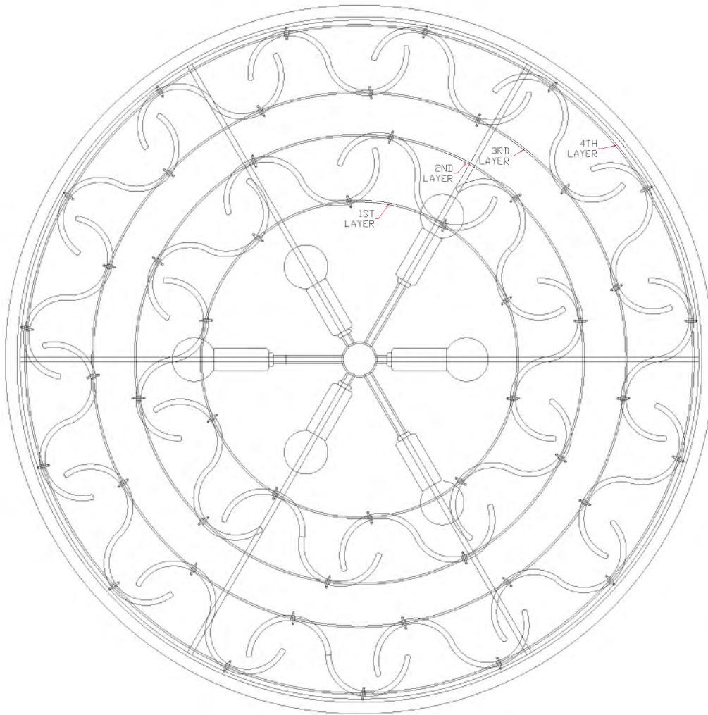
BOTTOM VIEW
