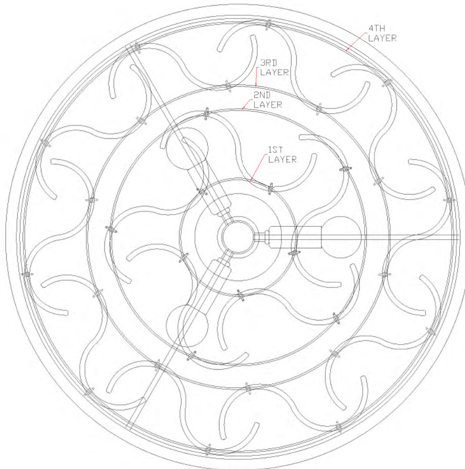
BOTTOM VIEW
