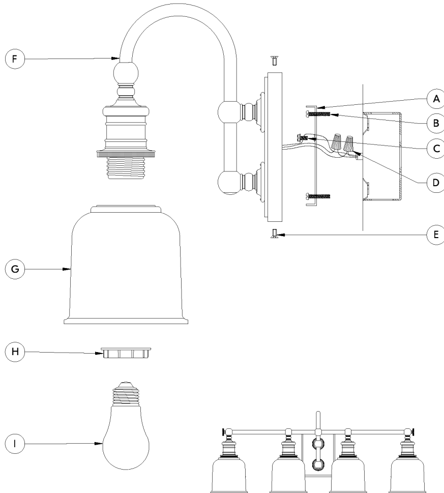
Front Elevation
