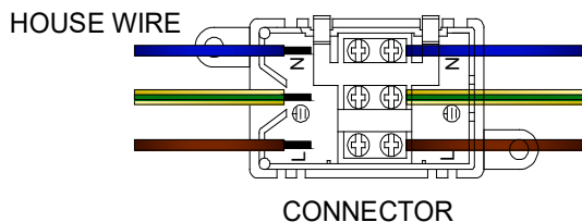
CONNECTOR
