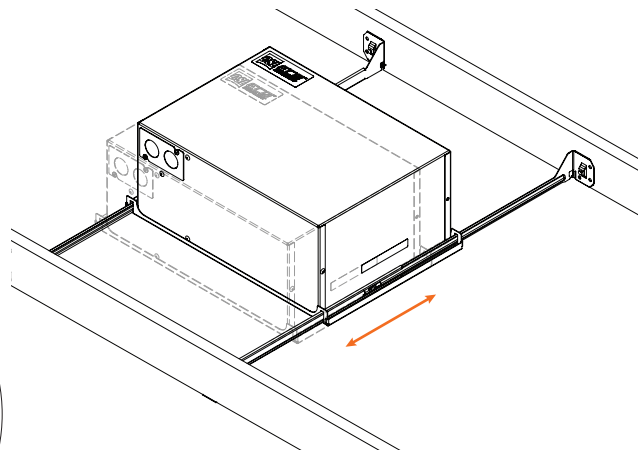
AIC Model
