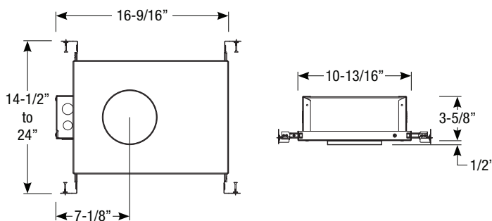
Field Cuttable Ceiling Cut-out: 5-1/8" Ø
