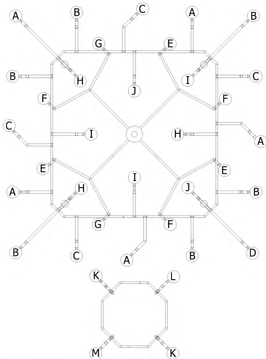
TOP VIEW OF THE FIXTURE
